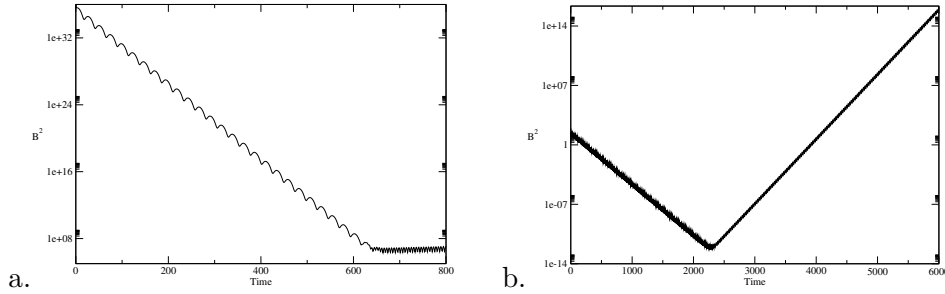
Figure 4.2 – Time evolution of the magnetic energy, which highlights the information provided by transient behaviours. Left (a) a simulation for R_m = 16.5 (< R_{m1}) using as initial condition the final solution obtained at R_m > R_{m1} , right (b) simulation for R_m = 28.4 (> R_{m1}) .
