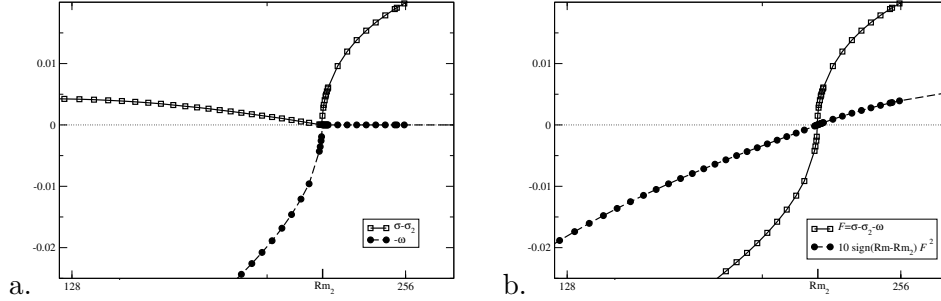
Figure 4.6 – Eigenvalues coalescence for R_m close to R_{m2} \simeq 215 . Both the real part (written as \sigma(R_m) - \sigma_2 ) and the opposite of the imaginary part (i.e. -\omega(R_m) ) are represented (a). The sum F of both (b), and \text{sign}(R_m - R_{m2})F^2 illustrate the continuity and regularity in the functional form of the eigenvalue (see text).
