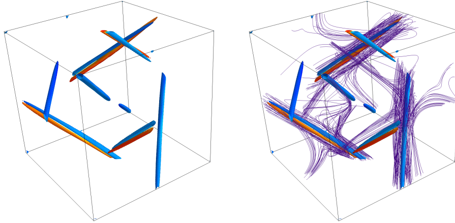
Figure 4.8 – Eigenmode obtained for R_m = 434.2 (> R_{m2}) . An isosurface of the magnetic energy is represented. To highlight the symmetry, it is coloured according to the value of B_x , from negative (dark gray - blue online) to positive (lighter gray - red online). The corresponding eigenvalue is purely real, yet the double cigars structure of the field remains clearly visible. Magnetic field lines are also depicted on the right plot.
